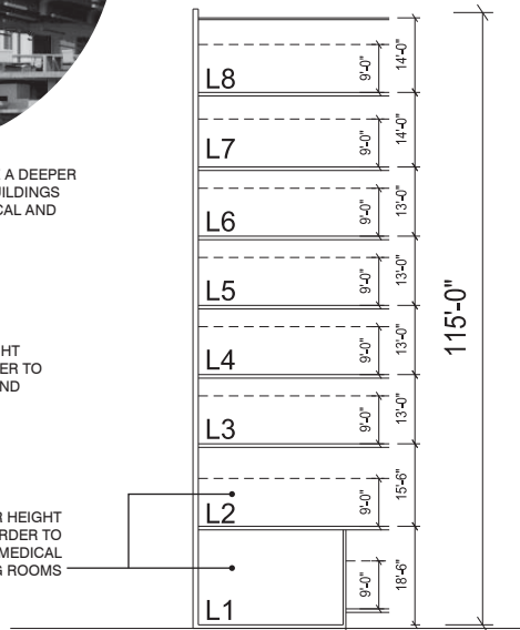
8 STORY HEALTH CARE FACILITY (AS PROPOSED)
